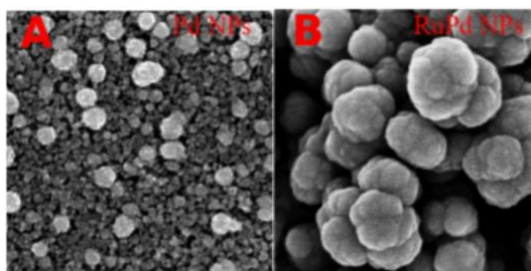
Figure 1. (A) FESEM image of Pd nanoparticles (Pd NPs) and (B) FESEM image of RuPd bimetallic nanoparticles (RuPd NPs) prepared by introducing 0.40 mM \text{RuCl}_3 \cdot x\text{H}_2\text{O} precursor into the original growth solution, showing modified morphology compared to monometallic Pd NPs.
